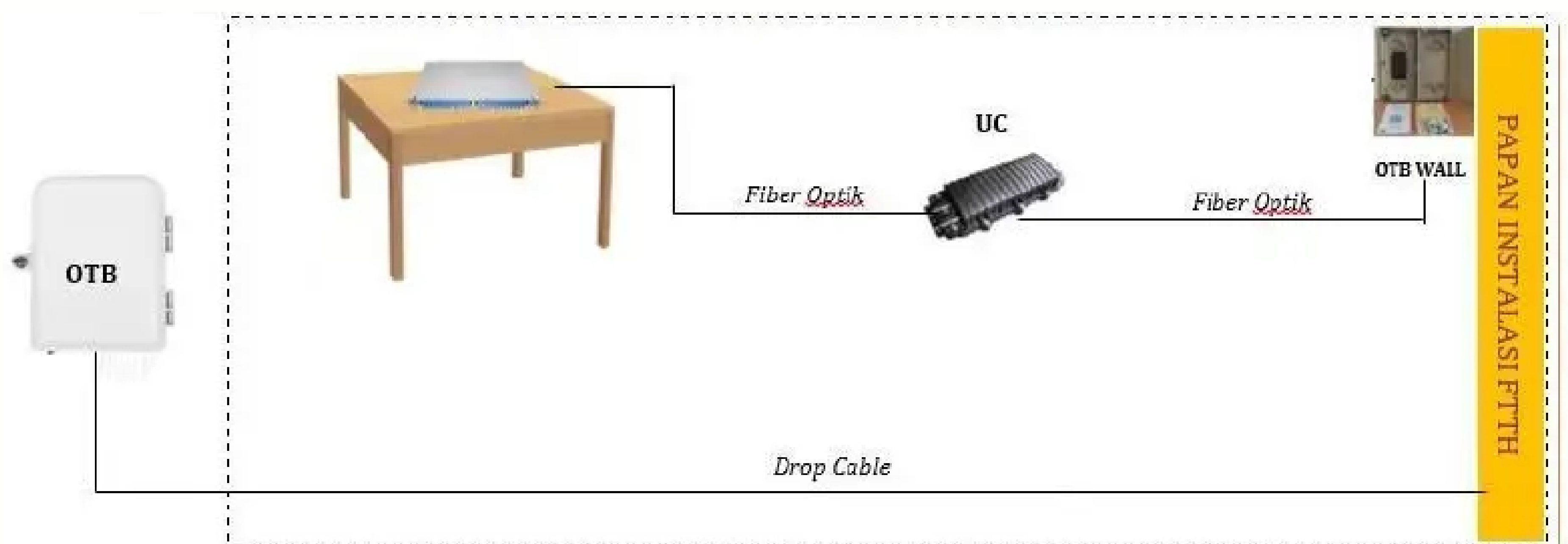
Gambar 2. Layout instalasi HRB
