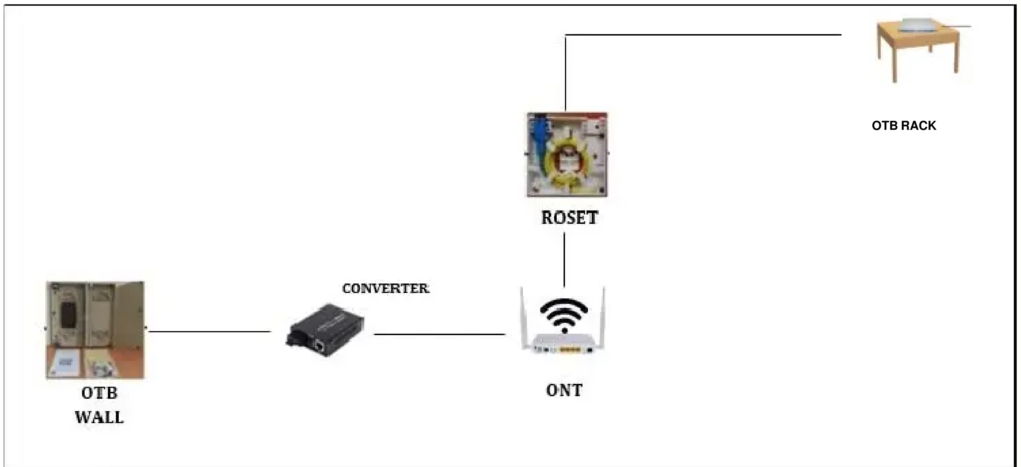
Gambar 3. Layout instalasi FTTH
